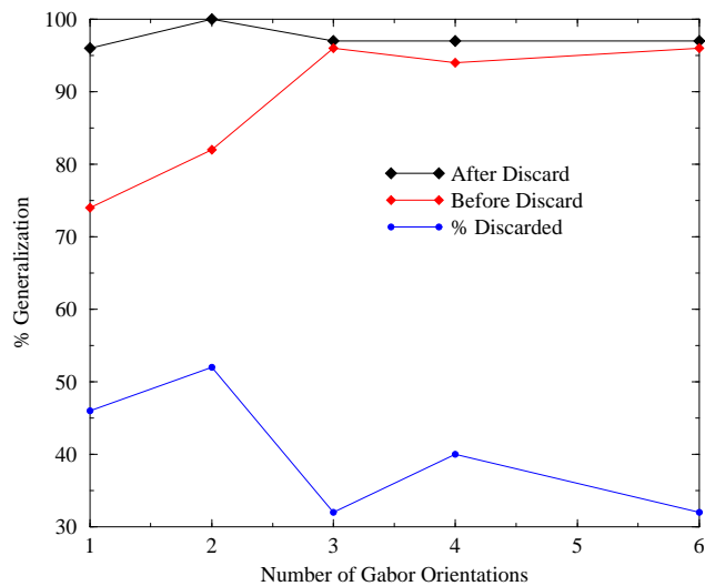
Figure 3.4. Effect of changing number of orientations on test generalisation and discard rates using Gabor Bx preprocessing of 1 \times 1
