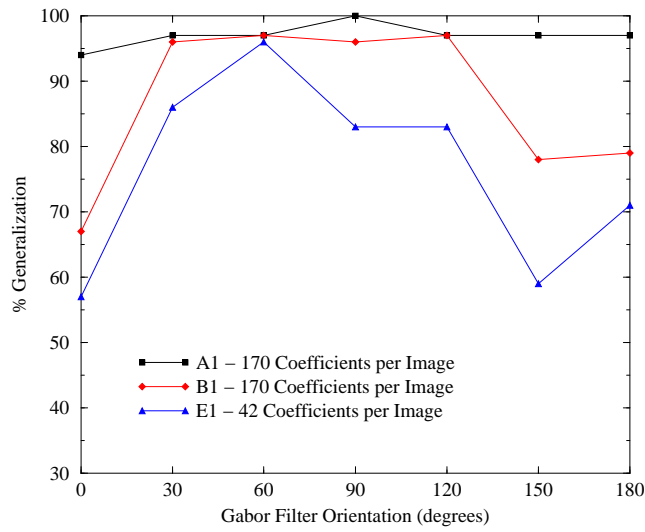
Figure 3.3. Effect of changing the angle of orientation in single orientation Gabor preprocessing on test generalisation after discard for 1 \times 1 RBF networks using 1 \times 1 face images from the Sussex database see Section C.1 Appendix C for details of sampling schemes
