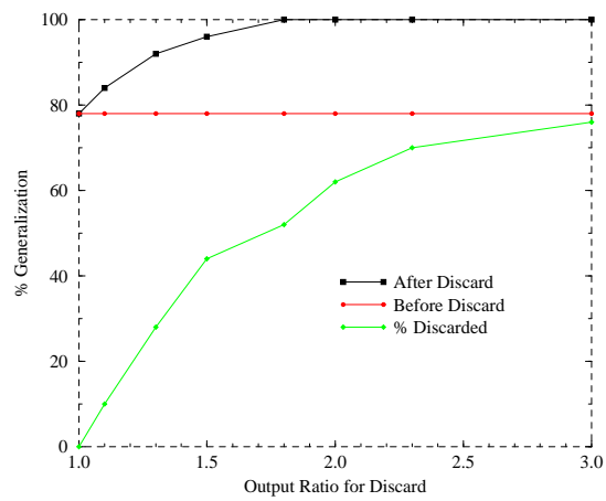
Figure 3.2.1 Effect on test generalisation after discard of changing the low confidence threshold for h_1 RBF networks trained with DoG preprocessed 1 \times 1 faces images from Sussex database. The low confidence threshold is based on the ratio between highest and second highest output units and a value of 1.5 has been found to be useful in practise.
