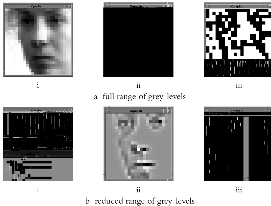
Figure C Effect of different ranges of grey levels for DoG preprocessing using a 16 \times 16 image i before preprocessing ii after non thresholded DoG preprocessing iii after thresholded DoG preprocessing
